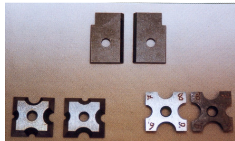
Quadruple and inner conductor stripping blades
